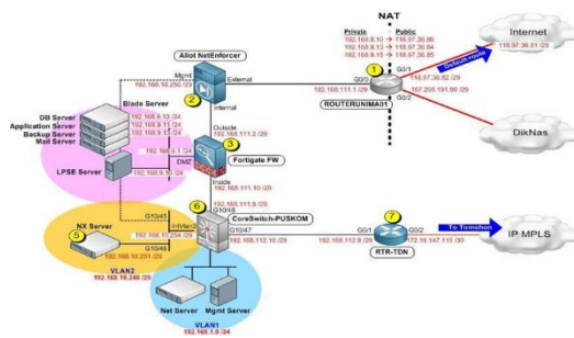
Gambar 3: Logical diagram (full view) jaringan kampus UNIMA
